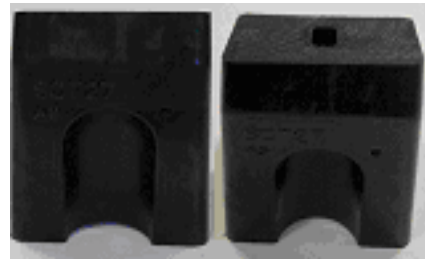
SCT-27 – 5400 Lb. Side Bearing Block For Use in 656-CRH, ISB-12 on 100 Ton Cars Needing More Hunting Control
