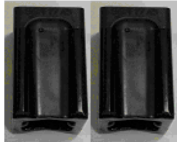
SCT-17 – 3000 Lb. Side Bearing Block For Use in 690-RL on Light 100 Ton Cars
